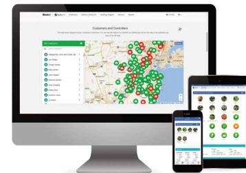
Hydrowise™ software
