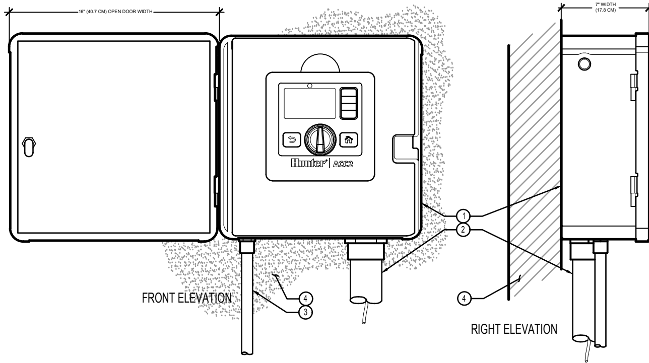
XX IRRIGATION CONTROLLER (ACC2) - METAL WALL MOUNT Hunter C.ACC2.01
