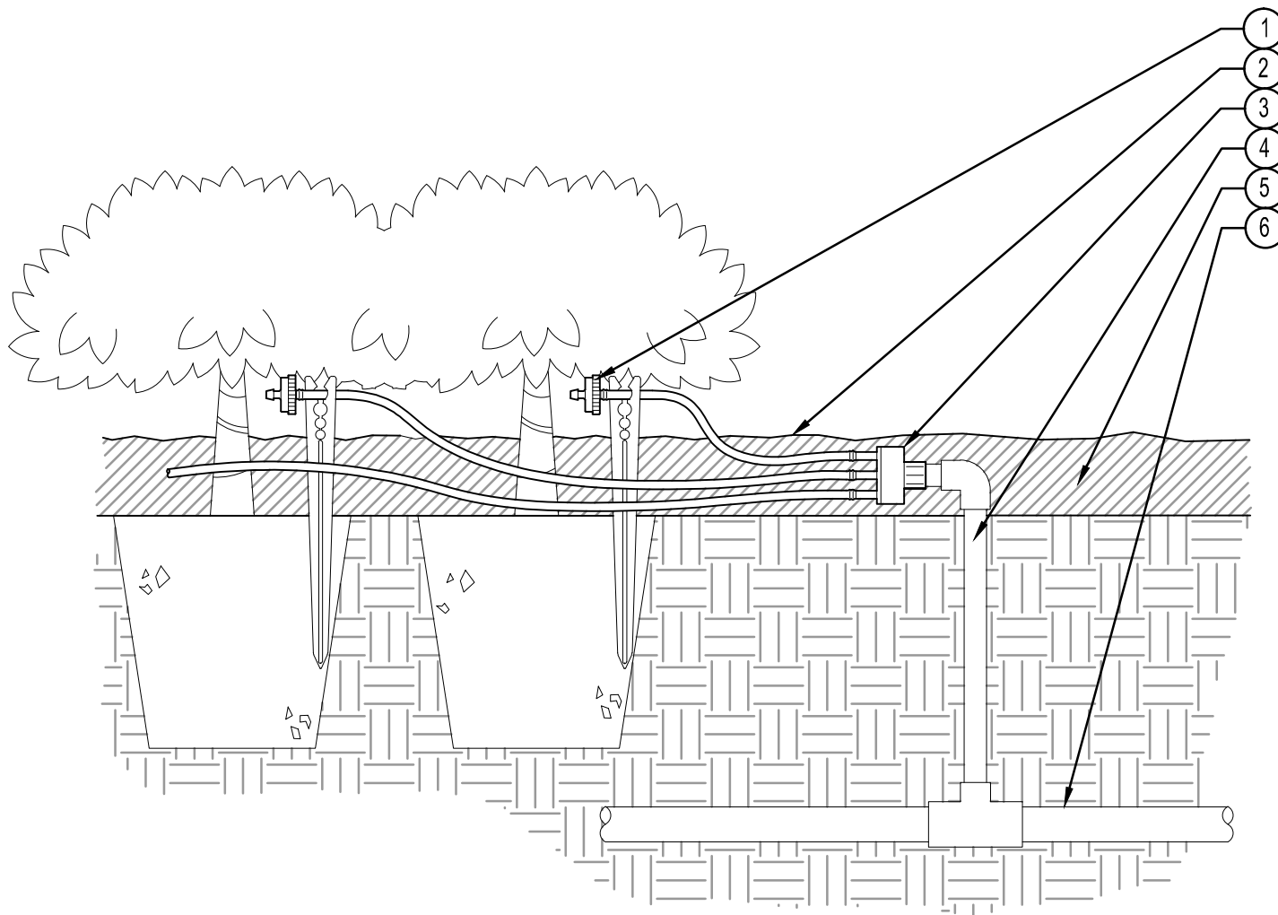
XX MULIT-PORT EMITTER - SIDE OFF PVC Hunter HM.MPM.02
