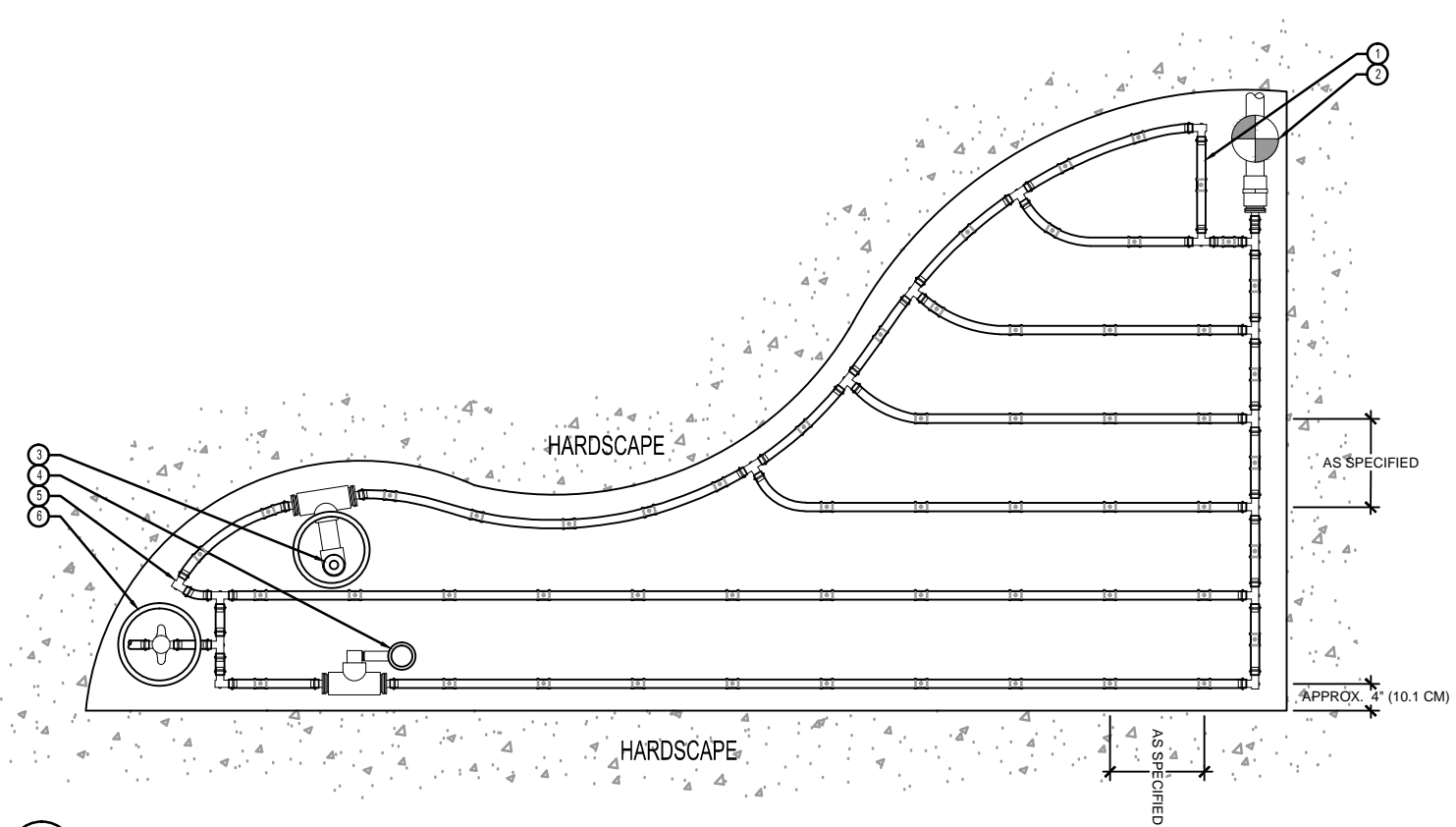
XX PROFESSIONAL LANDSCAPE DRIPLINE - IRREGULAR PLANTED AREA HM.PLD.02
