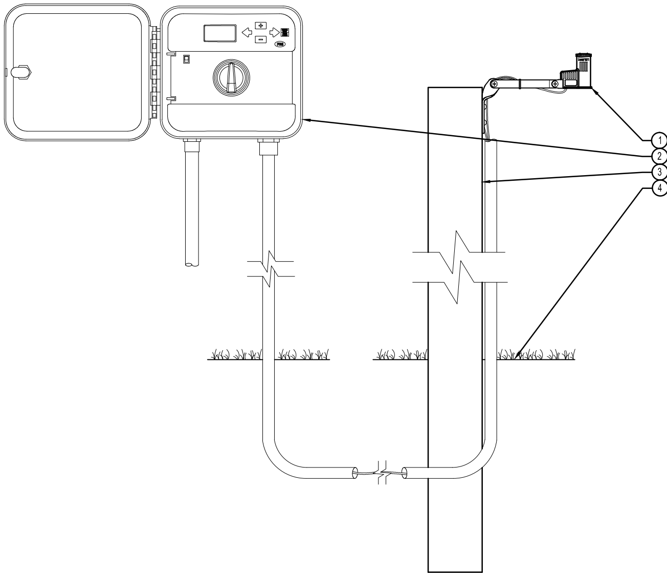
XX RAIN-CLIK WITH GENERIC WALL MOUNT CONTROLLER Hunter S.RC.01
