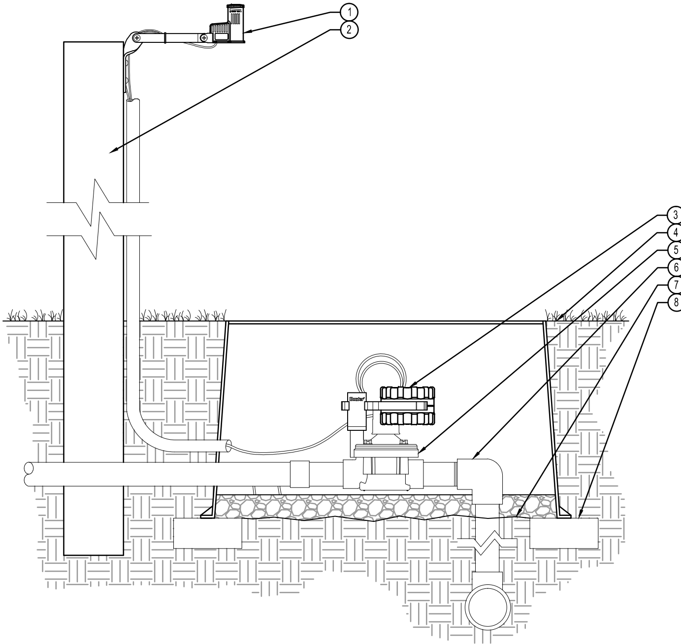
XX RAIN-CLIK WITH NODE CONTROLLER Hunter C.RC.03
